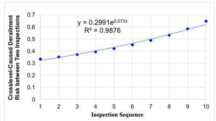
Figure 4 Track geometry caused derailment risk by traffic volume
