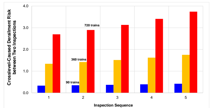
Figure 5 Derailment risk by traffic volume
